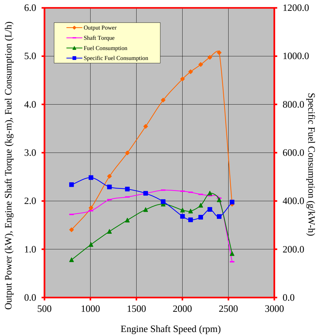
Figure 3. Performance characteristic curves of the KUBOTA RK70-S Diesel engine
