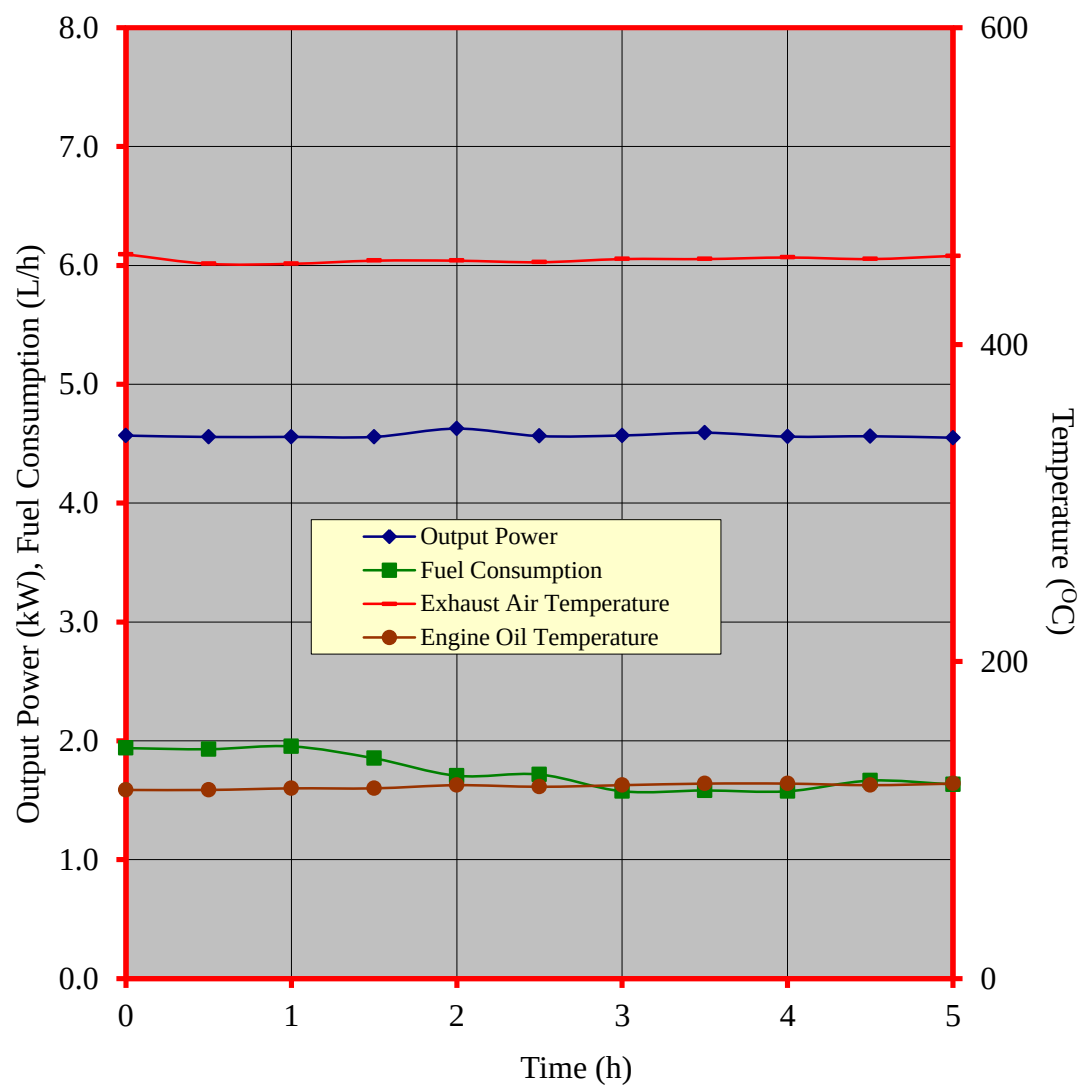
Figure 4. Performance characteristic curves during the continuous running test of the KUBOTA RK70-S Diesel Engine
